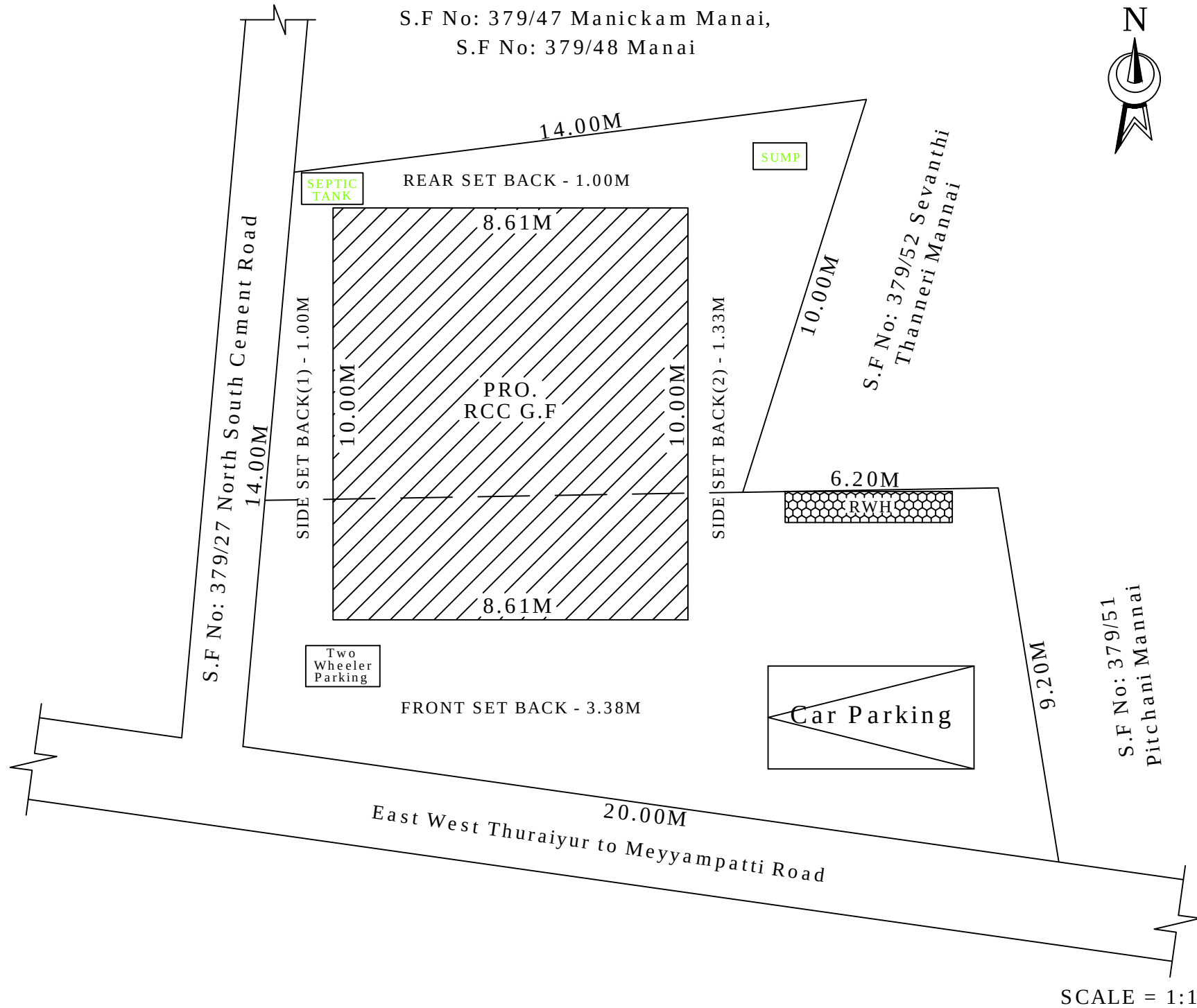
SITE PLAN
