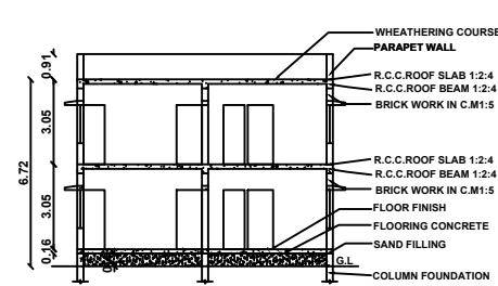
SECTION ON GG
