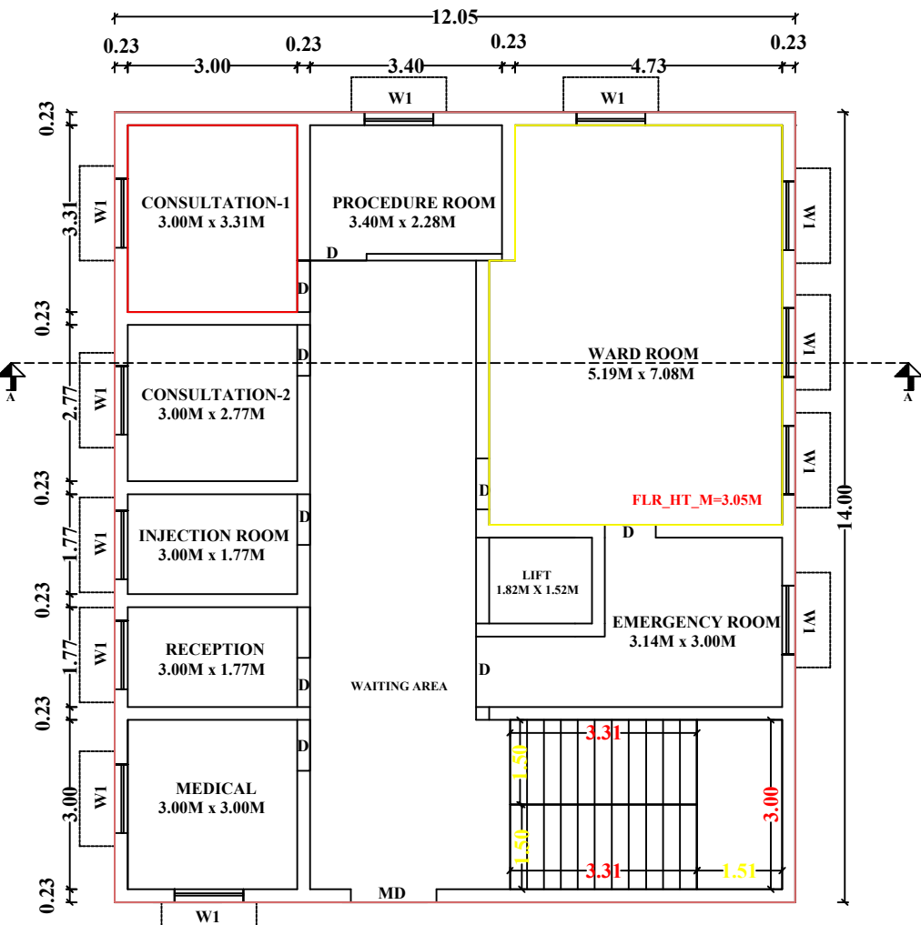
FLOOR-0
