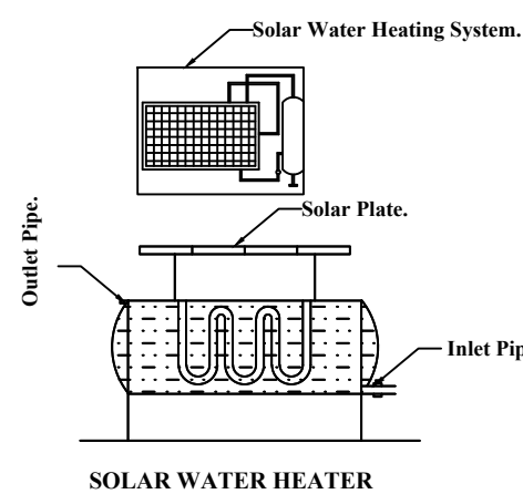
SOLAR WATER HEATER
