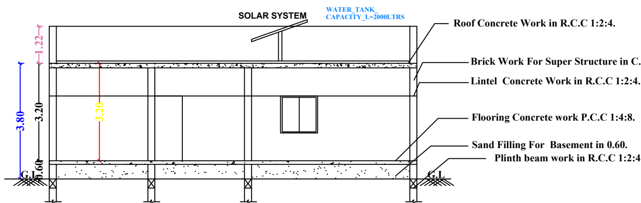
SECTION-AB
