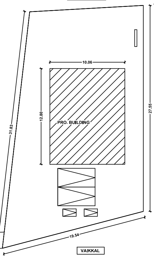
SITE PLAN
