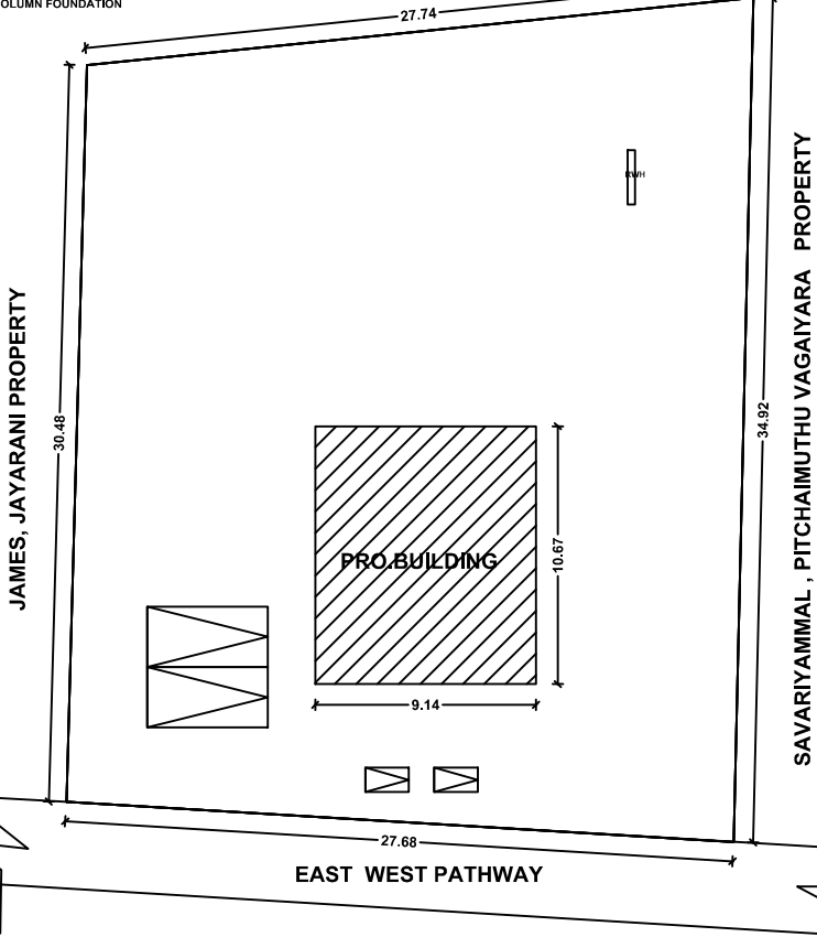
SITE PLAN
