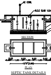
SEPTIC TANK DETAILS
