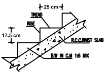
SECTION OF STAIRCASE
