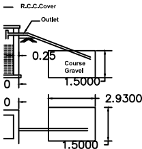
SEPTIC TANK & D-TRENCH DETAILS
