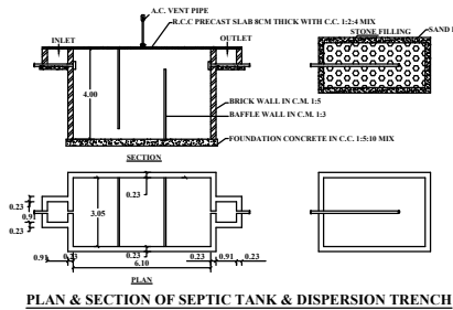
PLAN & SECTION OF SEPTIC TANK & DISPERSION TRENCH
