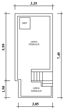
GROUND FLOOR ROOF
