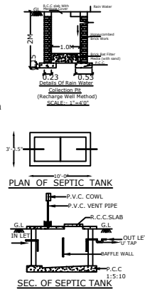
SEC. OF SEPTIC TANK
