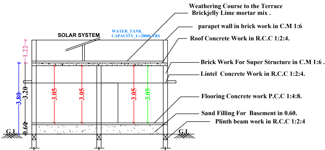
SECTION-AB
