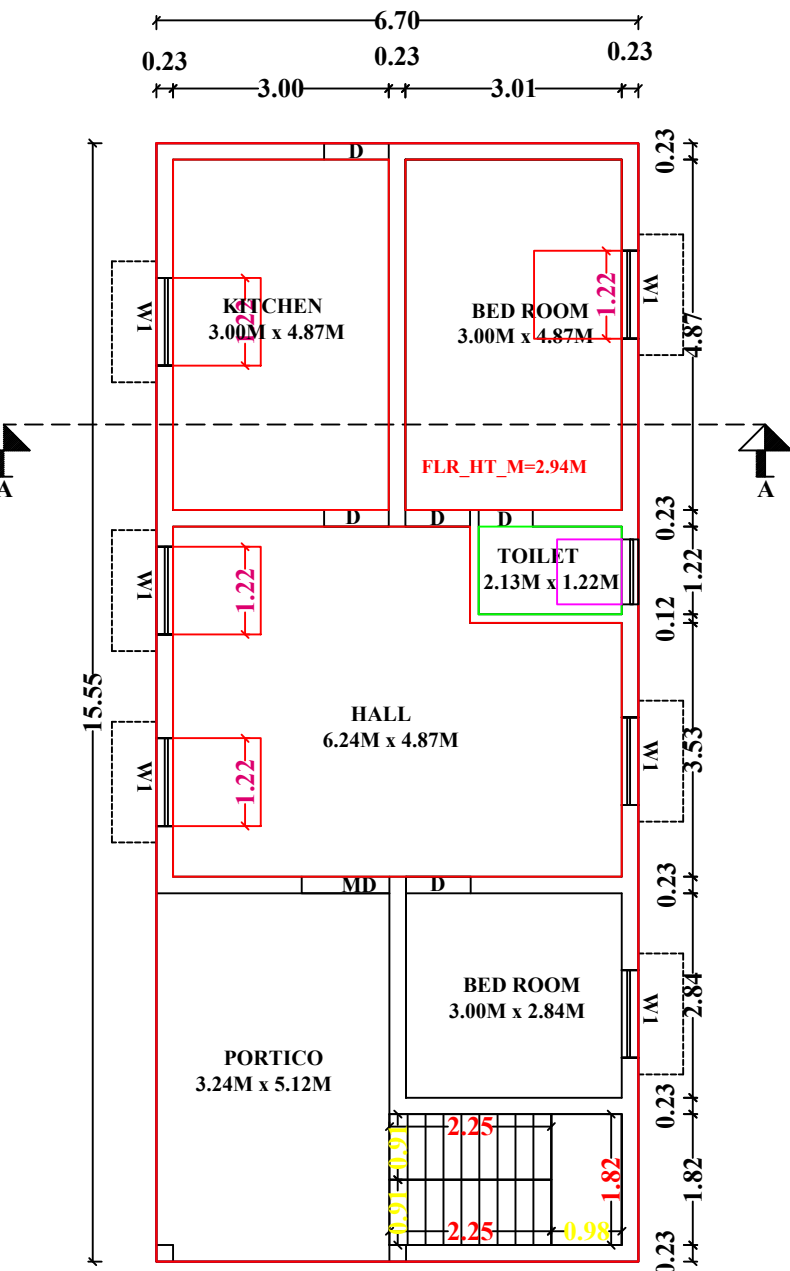
FLOOR-0
