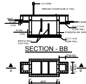
RAIN WATER TANK
