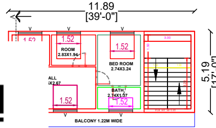
POSED FIRST FLOOR PLAN
