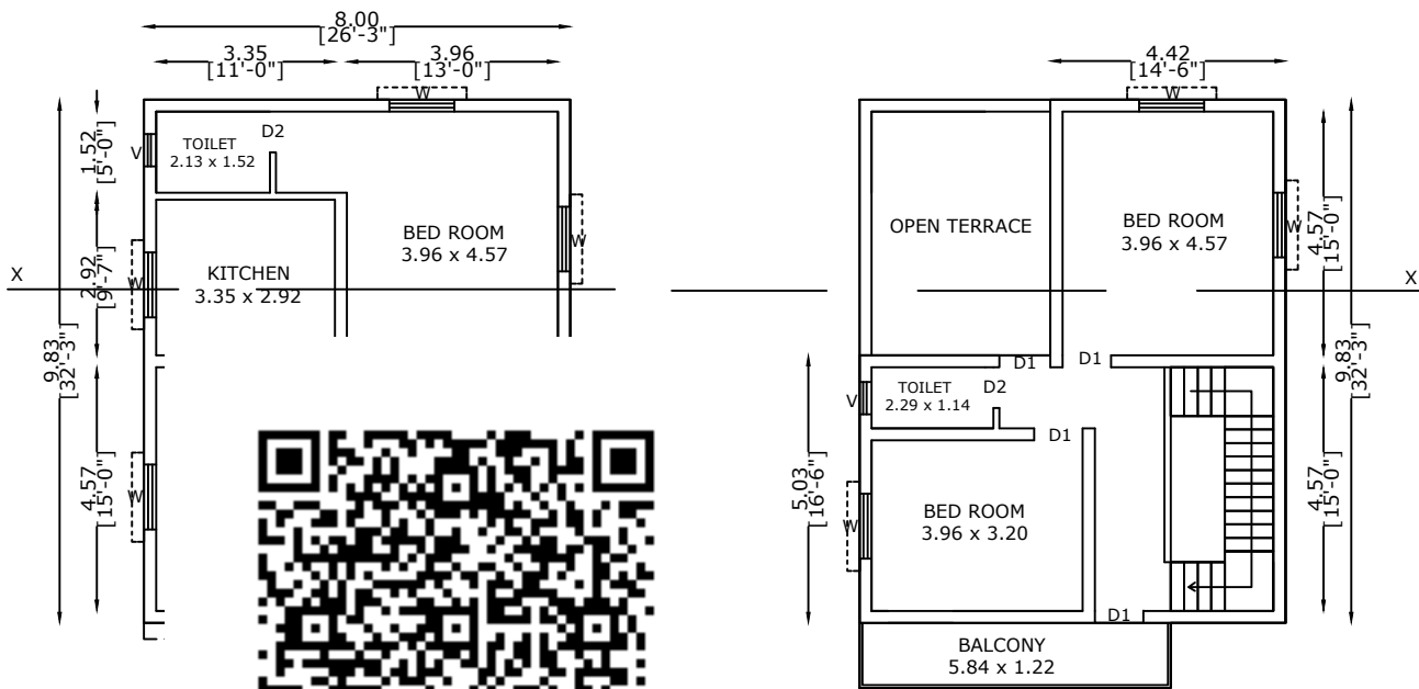
PRO. FIRST FLOOR PLAN
