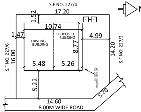
SITE PLAN
