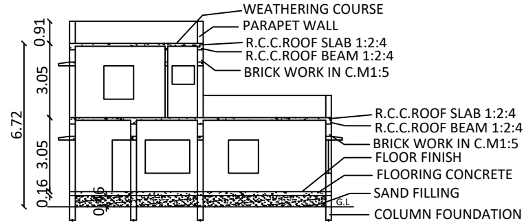
SECTION- SS
