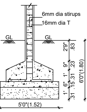
COLUMN FOUNDATION DETAIL SCALE (1:50)
