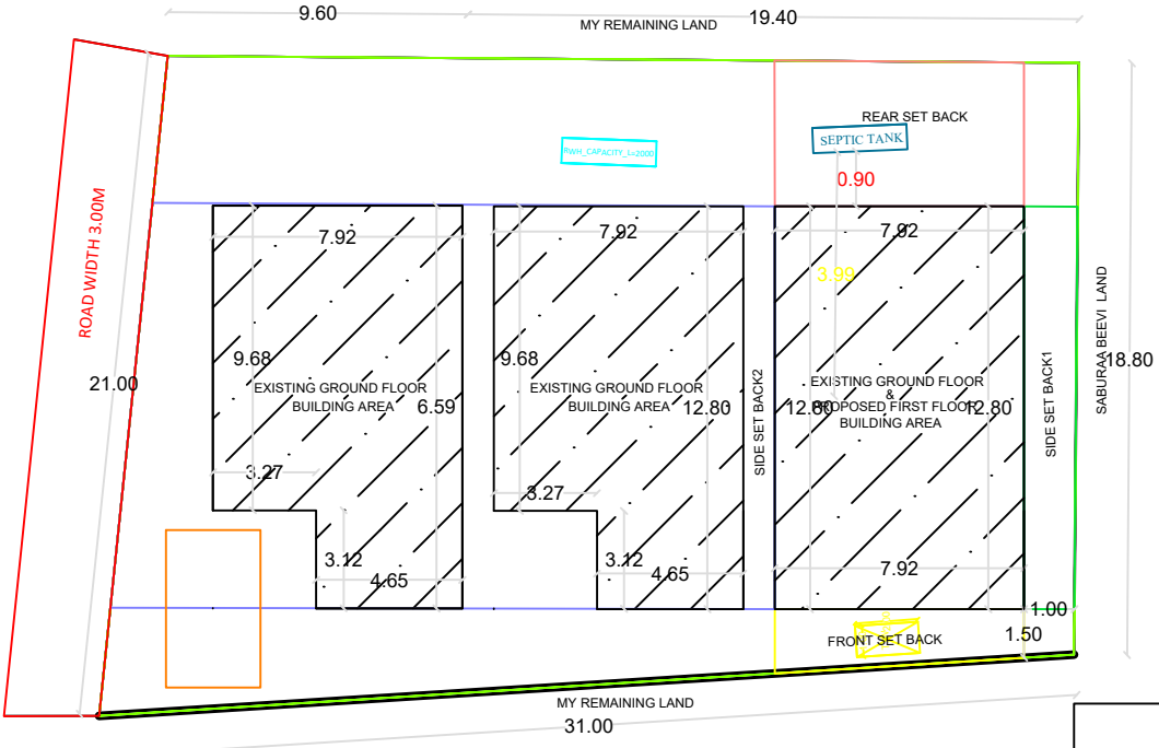
SITE PLAN
