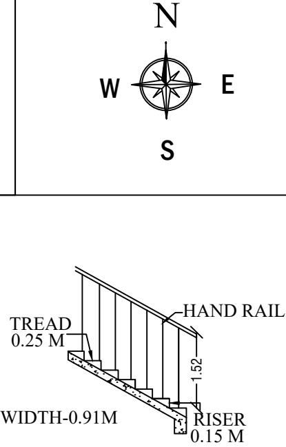
STAIRCASE DETAILS
