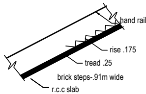
STAIR DETAILS
