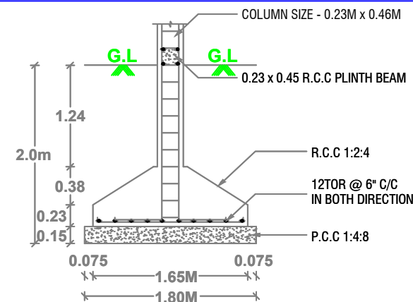
COLUMN FOOTING DETAILS - A Column 'C1' - 0.23m x 0.46m NOT TO SCALE
