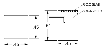
PLAN
