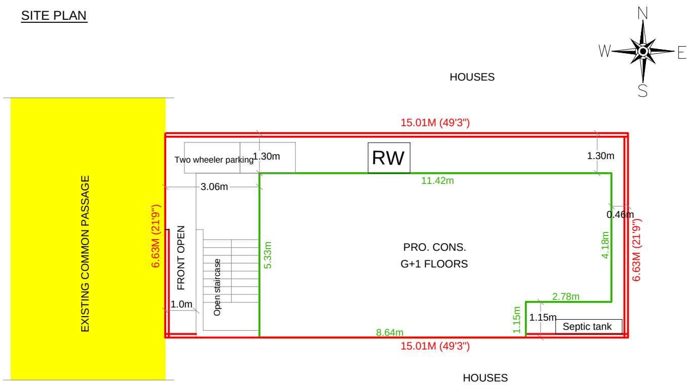
SITE PLAN
