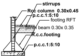
COLUMN DETAILS
