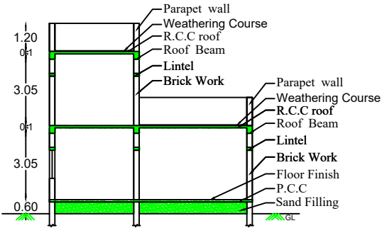
SECTION AB
