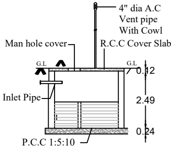
SECTION
