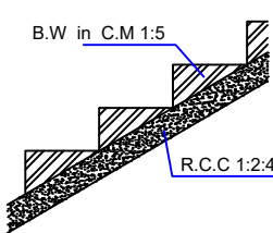
STAIRCASE
