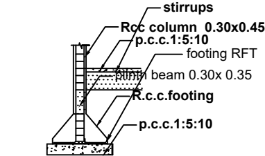
COLUMN DETAILS
