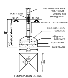
FOUNDATION DETAIL
