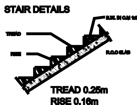
STAIR CASE
