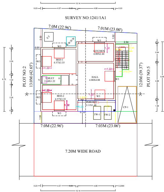
SITE PLAN CUM GROUND FLOOR PLAN
