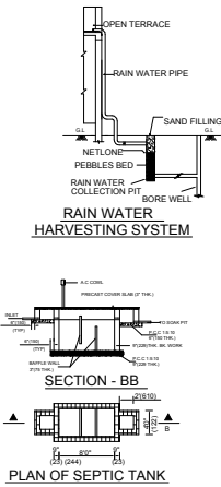
PLAN OF SEPTIC TANK
