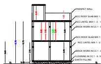
SECTION ON AB & ( HALF ELEVATION)
