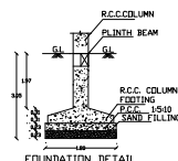
FOUNDATION DETAIL
