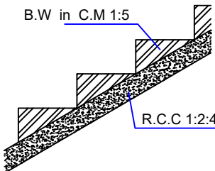
STAIRCASE
