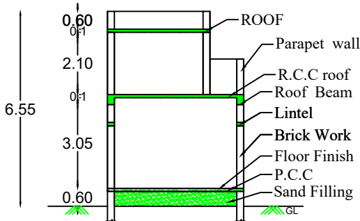
SECTION AB
