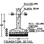
FOUNDATION DETAIL
