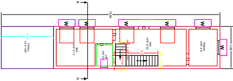
GROUND FLOOR
