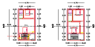
PRO GROUND FLOOR PLAN
