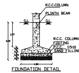
FOUNDATION DETAIL
