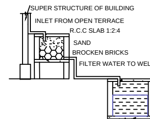
RAINWATER HARVESTING
