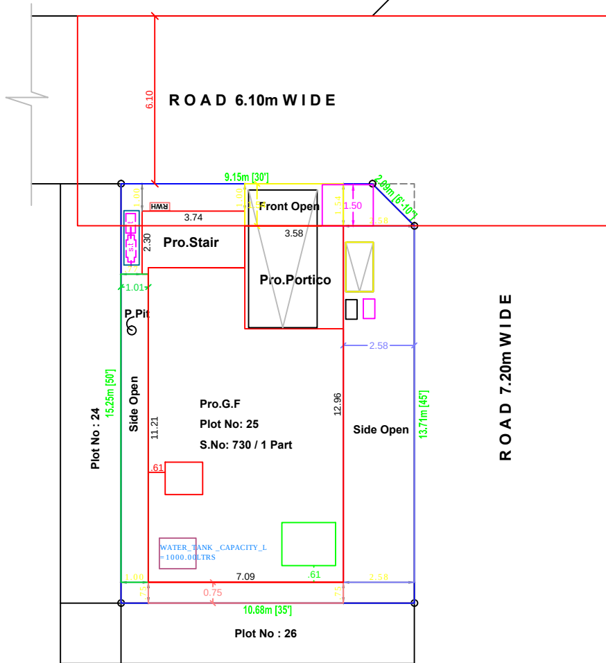
SITE PLAN
