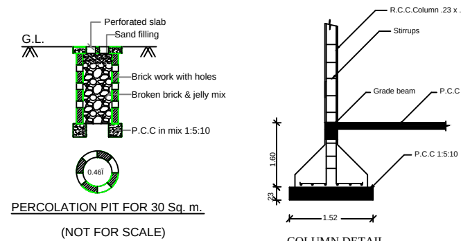
COLUMN DETAIL
