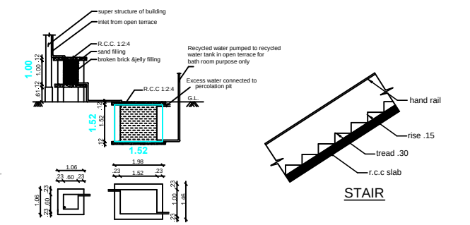
STAIR
