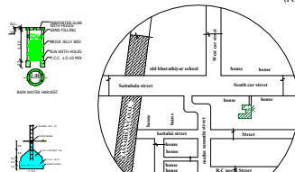
LOCATION PLAN (NOT TO SCALE)
