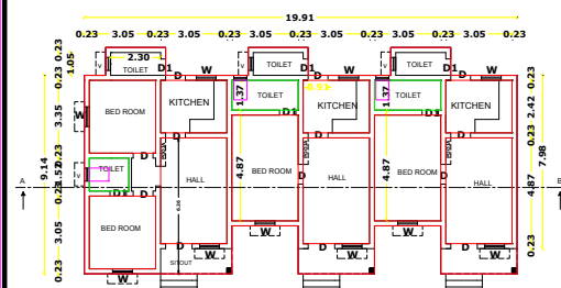
PROPOSED GROUND FLOOR PLAN SCALE 1:100
