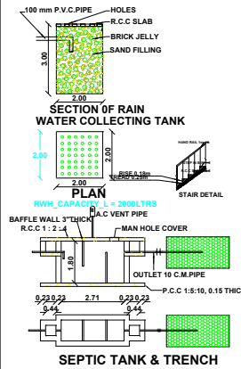
SEPTIC TANK & TRENCH
