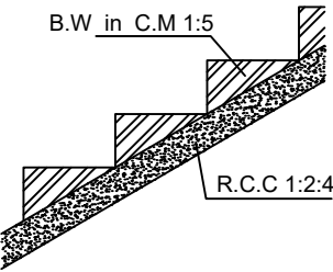
STAIRCASE
