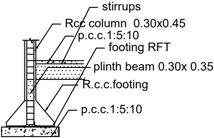
COLUMN DETAILS
