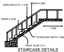
STAIRCASE DETAILS
