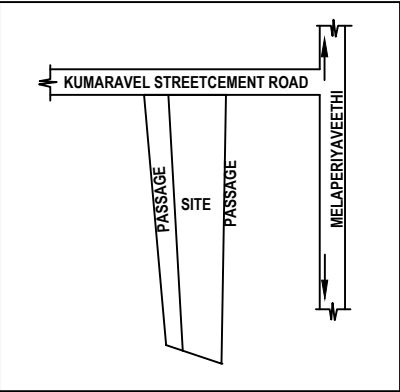
LOCATION PLAN
