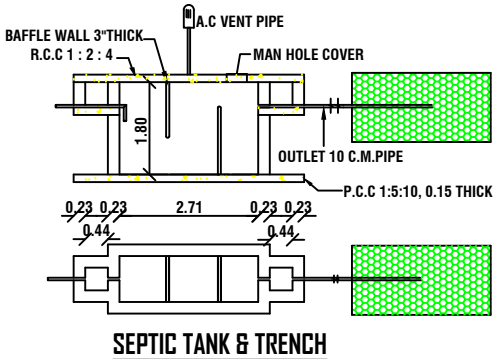
SEPTIC TANK & TRENCH
