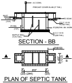
SECTION - BB PLAN OF SEPTIC TANK
