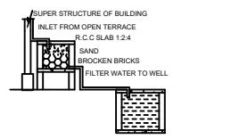
RAINWATER HARVESTING
