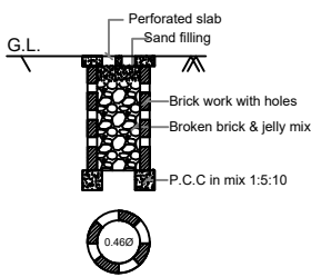
PERCOLATION PIT FOR 30 Sq. m.
