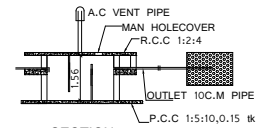
SECTION PLAN OF SEPTIC TANK & TRENCH
