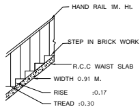
STAIR DETAIL
