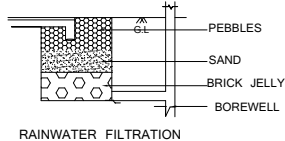
RAINWATER FILTRATION
