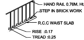
STAIR CASE DETAIL
