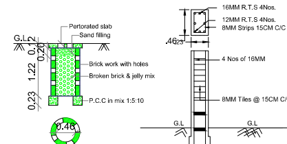
PERCOLATION PIT (Scale:- 1:50)
