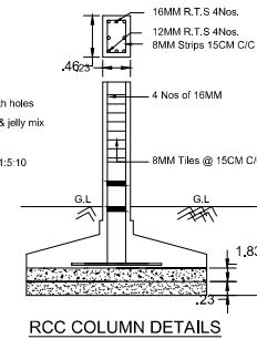
RCC COLUMN DETAILS
