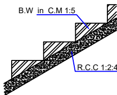
STAIRCASE
