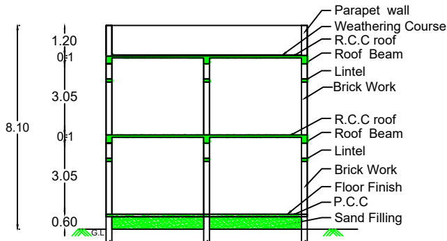
SECTION AB
