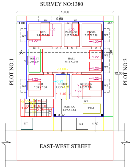
SITE PLAN CUM GROUND FLOOR PLAN
