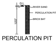
PERCOLATION PIT
