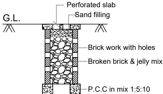
RAINWATER HARVESTING
