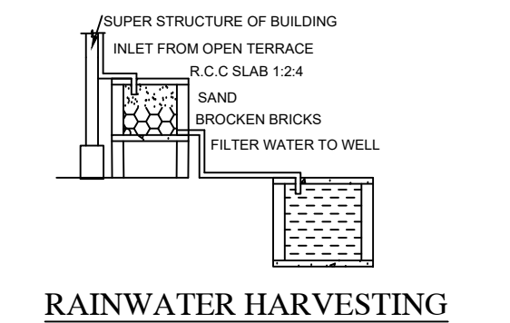
RAINWATER HARVESTING
