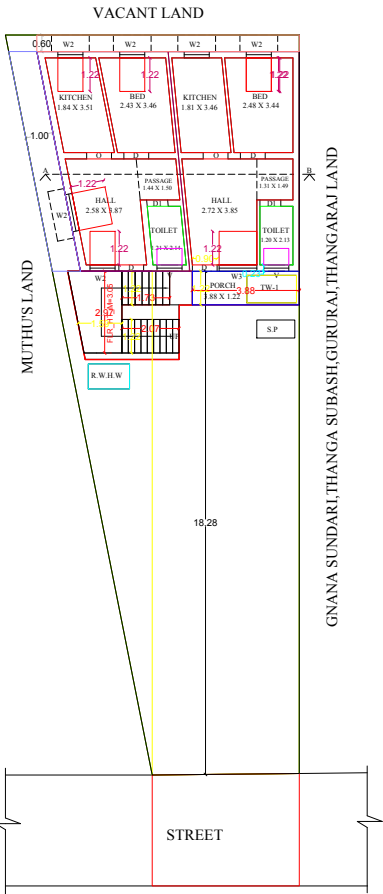
SITE PLAN CUM GROUND FLOOR PLAN
