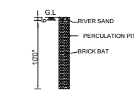
PERCOLATION PIT
