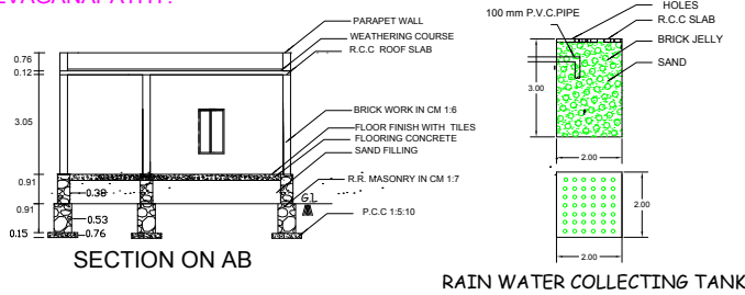
RAIN WATER COLLECTING TANK
