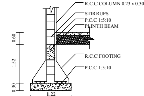
COLUMN DETAILS
