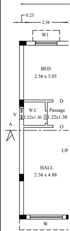
GROUND F
