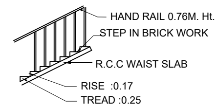
STAIR CASE DETAIL
