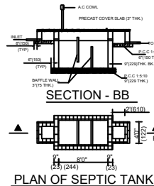
PLAN OF SEPTIC TANK
