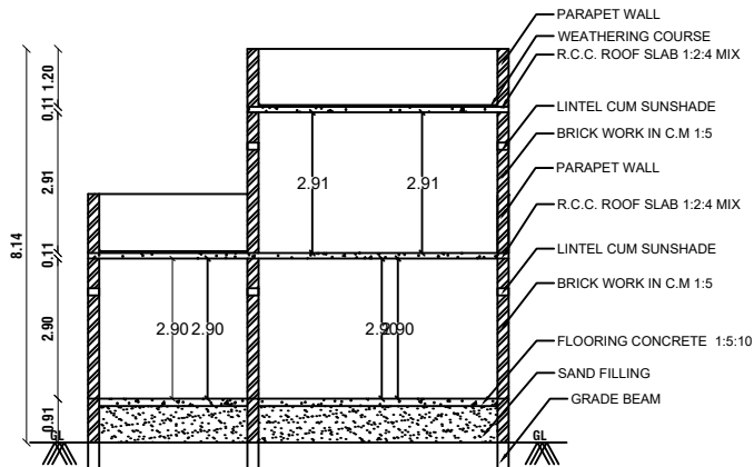
SECTION-AB
