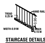
STAIRCASE DETAILS
