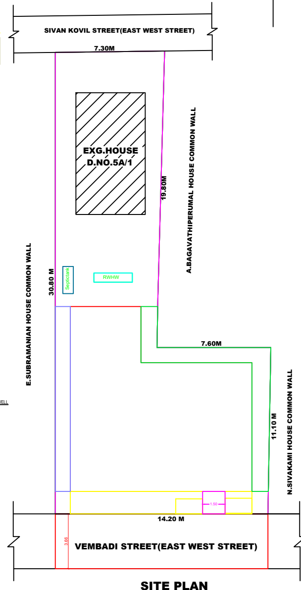
SITE PLAN
