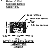
DETAILS OF RAIN WATER HARVESTING Dwg-1A
