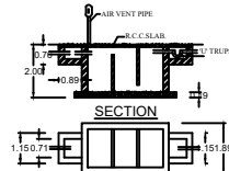
SEPTIC TANK PLAN
