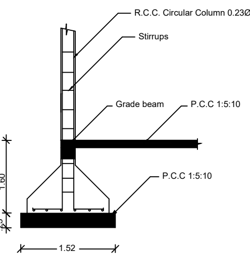
COLUMN DETAIL
