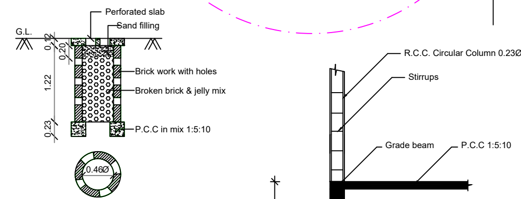
PERCOLATION PIT FOR 30 Sq.m. (scale:- 1:50)
