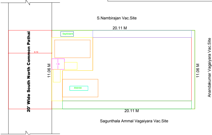
SITE PLAN
